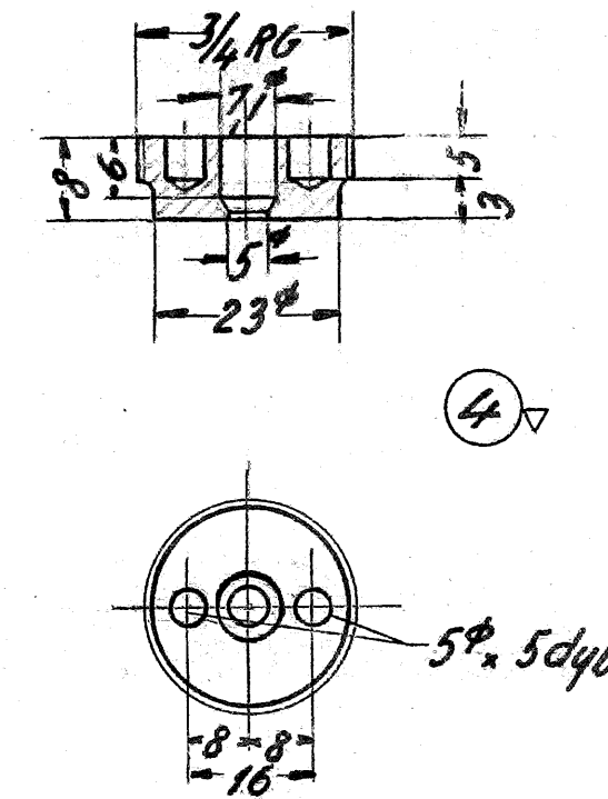
4 bundstyr 3/4" RG x 8 metal
